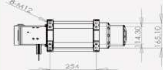
XRC 15 Mounting Pattern
