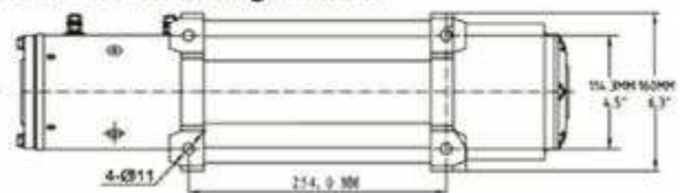
XRC 10 Mounting Pattern
