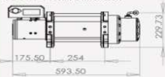
XRC 15 Mounting Pattern
